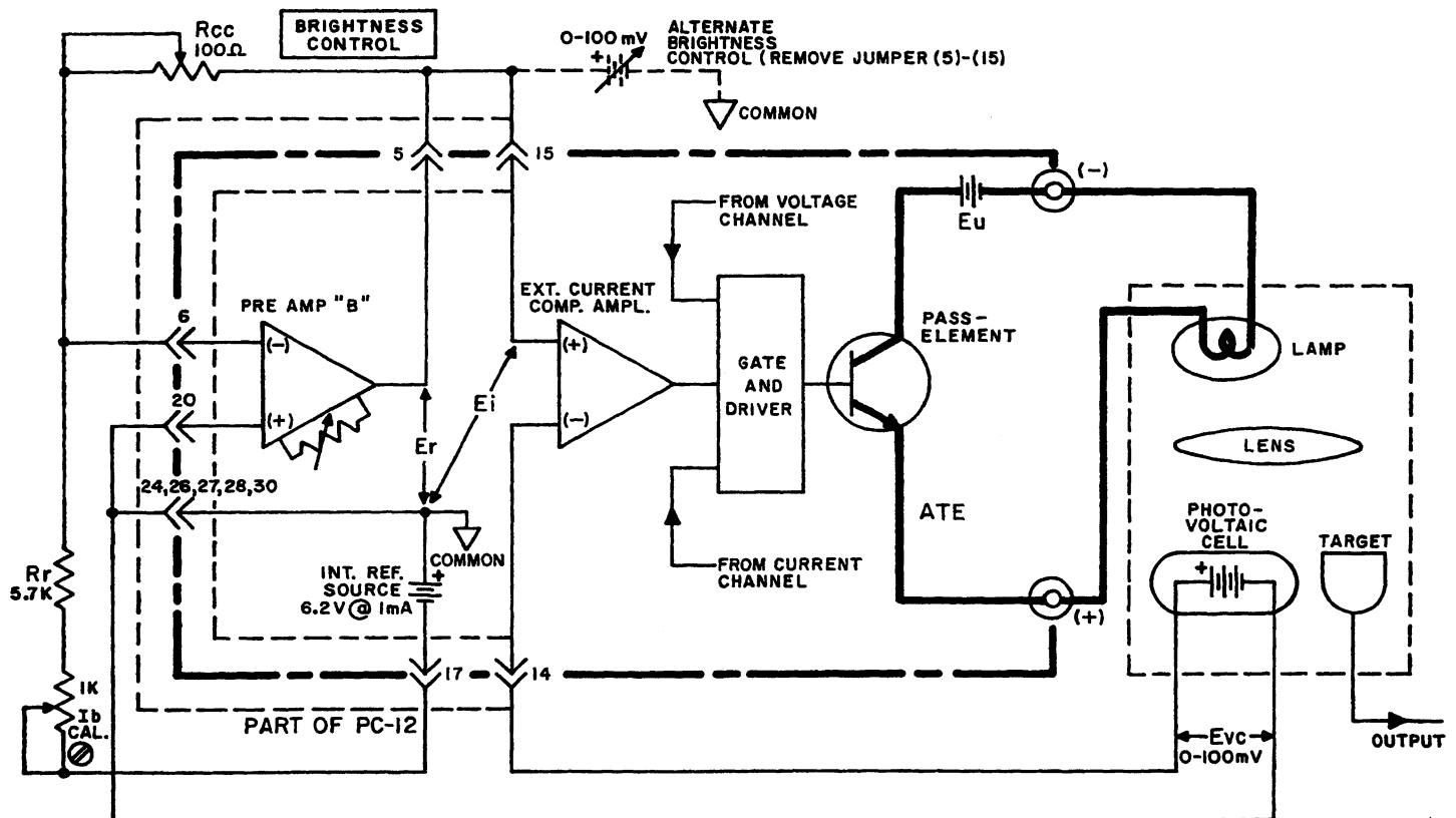
FIG. 3-17 ILLUMINATION CONTROL CIRCUIT WITH THE ATE POWER SUPPLY.
